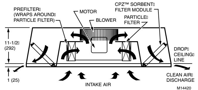
Fig. 9. F118 Air Cleaner operation.
