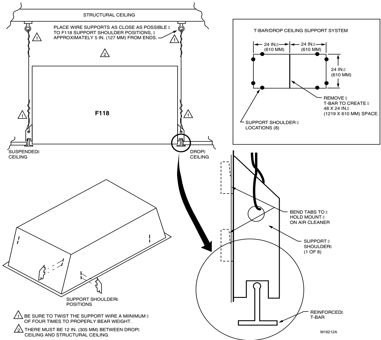
Fig. 4. Mounting procedure.
