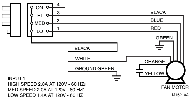
Fig. 5. Typical F118 120V, 60 Hz Wiring Diagram.
